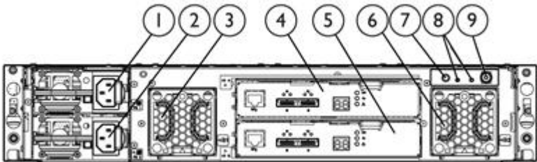
HPE D2700 Disk Enclosure Rear Panel components
