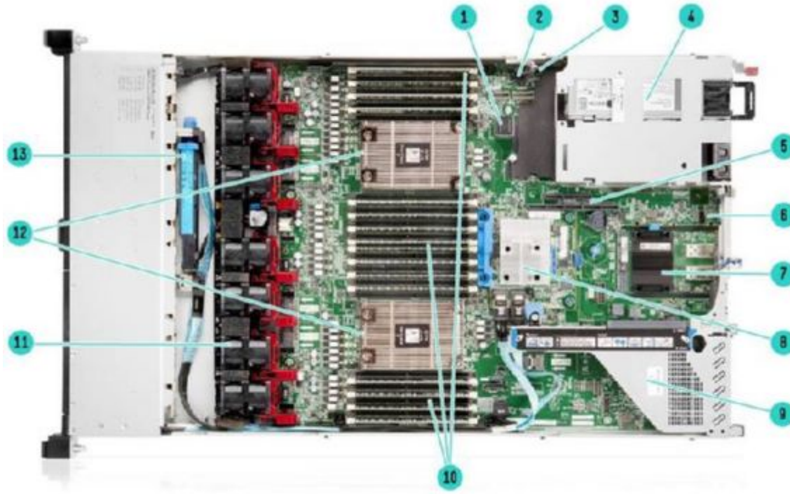
Internal View - Standard for all DL365 Gen10 Plus
