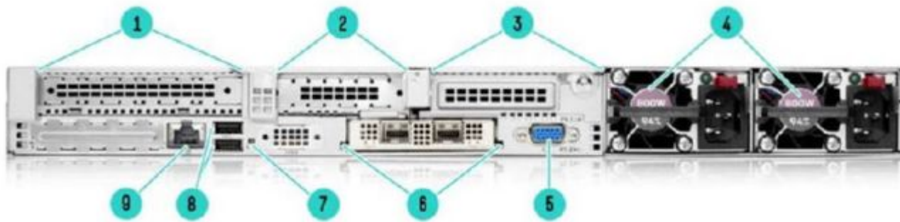
Rear View - Standard for all DL365 Gen10 Plus
